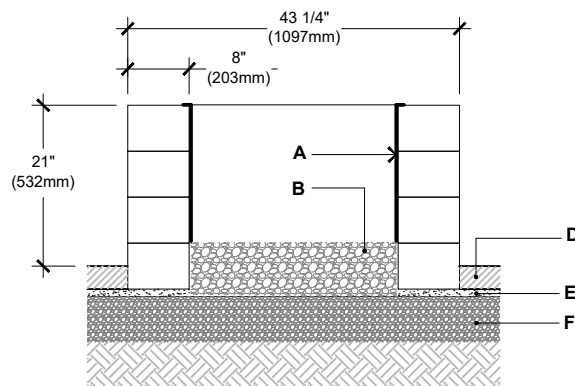
SECTION 1-1
