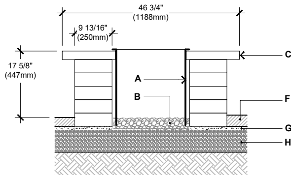
SECTION 1-1
