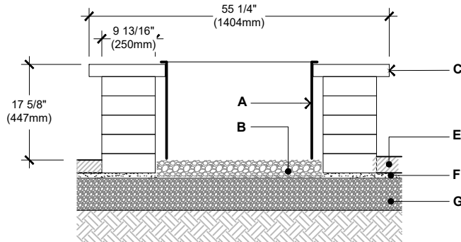
SECTION 1-1
