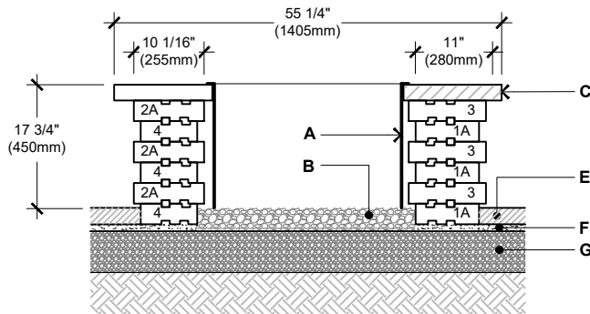
SECTION 1-1
