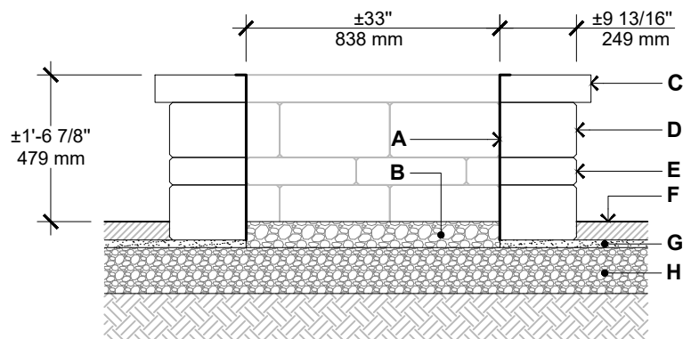
SECTION 1-1
