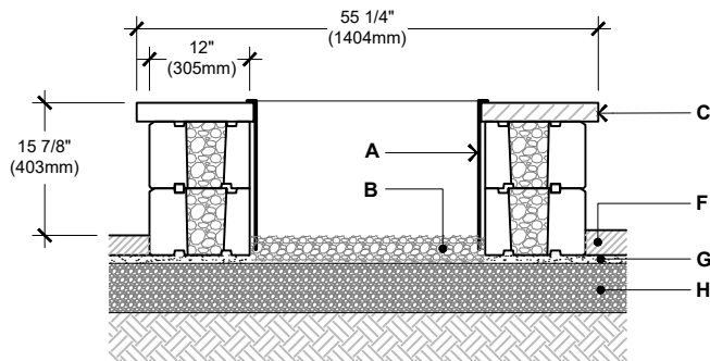
SECTION 1-1
